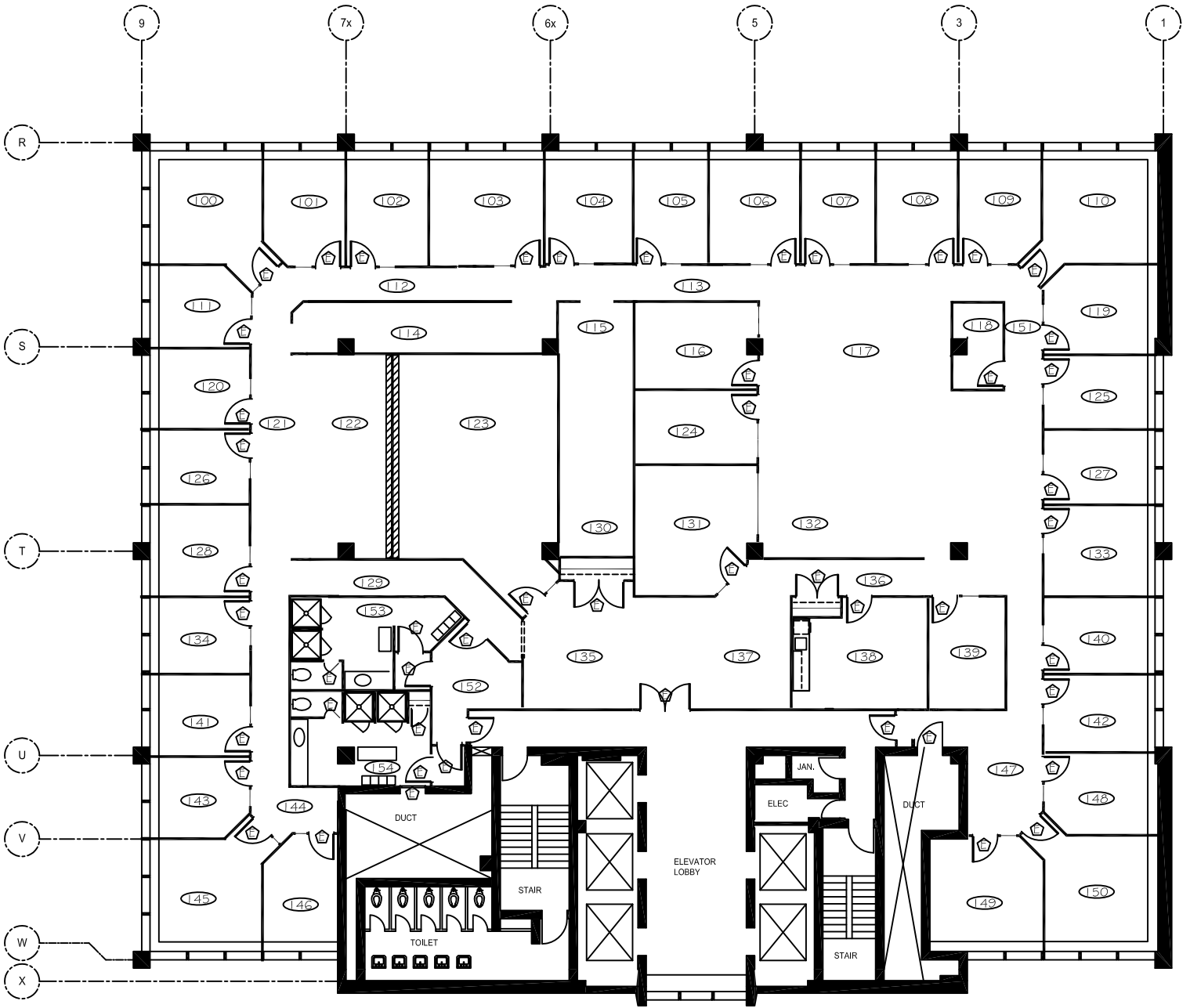
PLAN - DEMOLITION / NEW PARTITION SCALE: 1/8" = 1'-0"
